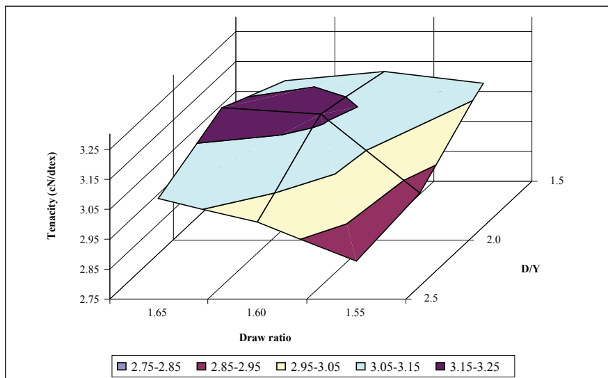
FIGURE 3. The influences of draw ratio and D/Y ratio on tenacity
