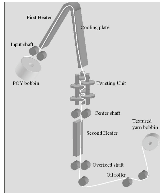
FIGURE 1. Barmag M profile false-twist texturing machine
