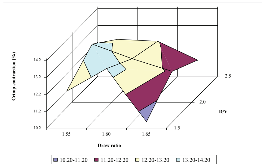
FIGURE 4. The influences of draw ratio and D/Y ratio on crimp contraction
