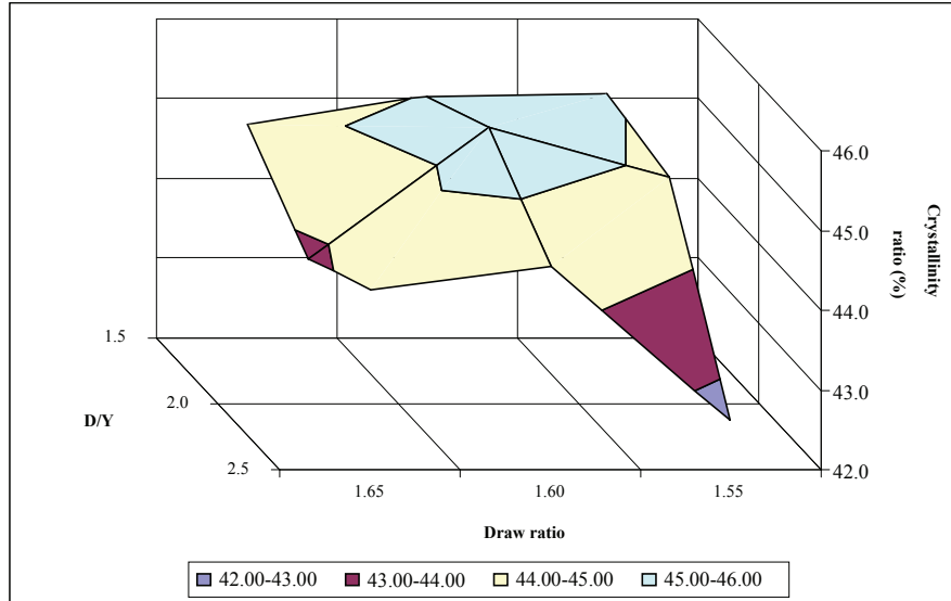
FIGURE 2. The influences of draw ratio and D/Y ratio on crystallinity ratio
