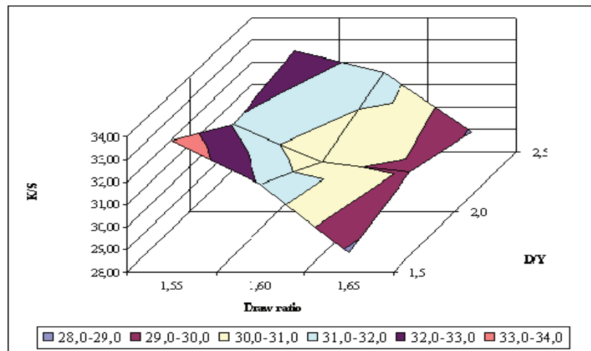
FIGURE 6. The influences of draw ratio and D/Y ratio on K/S
