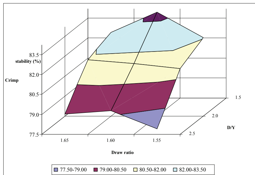
FIGURE 5. The influences of draw ratio and D/Y ratio on crimp stability
