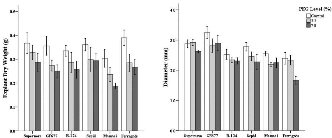
Figure 1. Effect of PEG induced drought stress on dry weight and diameter of almond genotypes explants.
