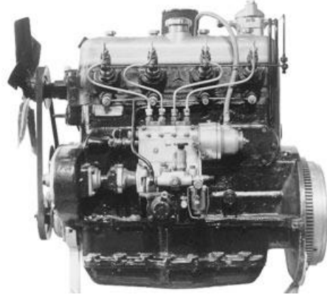
Şekil 2.1. Mercedes-Benz 260D motoru (BOSCH Diesel Motor Management 2002)
