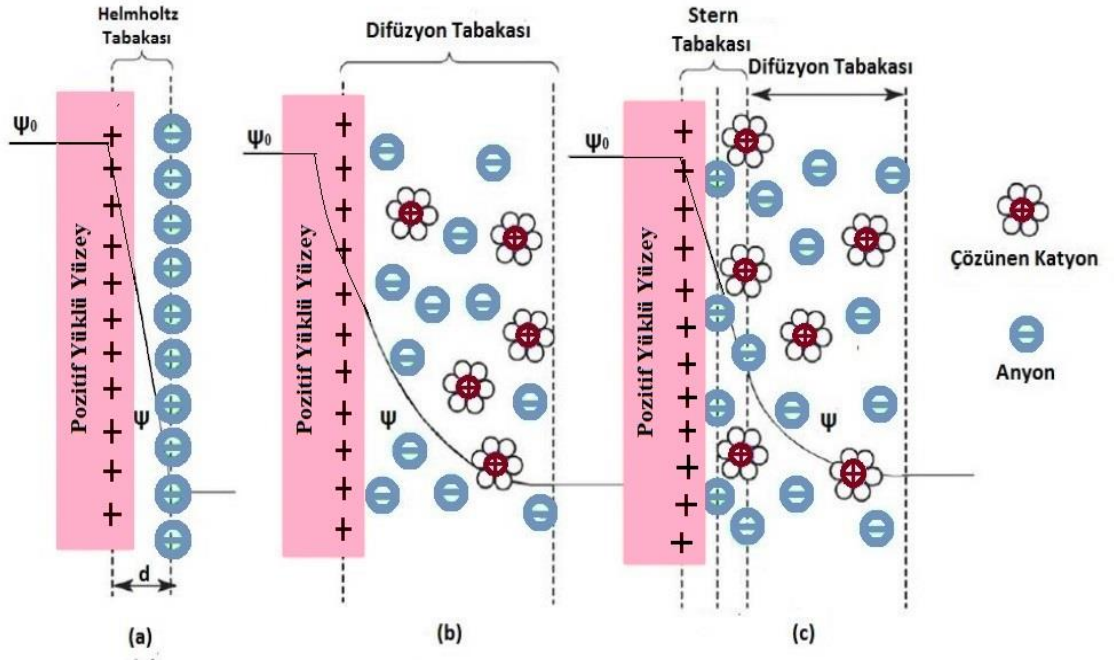
Şekil 2.6. (a) Helmholtz model (b) Gouy ve Chapman model (c) Stern model (Conway 1999)
